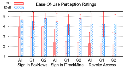
(a) The perceived ease-of-use Likert-scale ratings.
