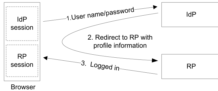
(a) The Web SSO system model.
