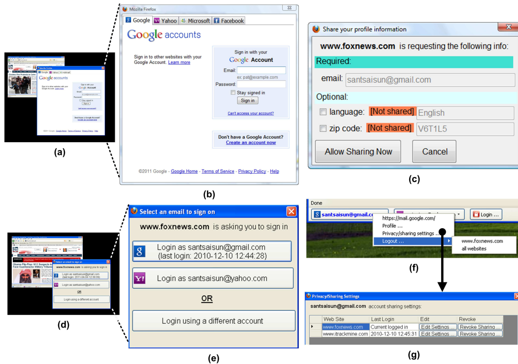
Fig. 4. Main screens of the identity-enabled browser (IDeB): (a) block-out desktop and IdP login form, (b) IdP login form that supports accounts from Google, Yahoo, Microsoft and Facebook, (c) profile sharing consent form, (d) block-out desktop and IdP account selector, (e) IdP account selector, (f) IdP identity indicator, (g) profile sharing setting form.
