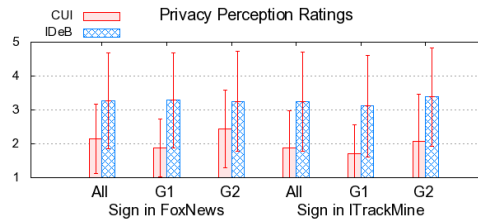
(c) The perceived privacy control Likert-scale ratings.
