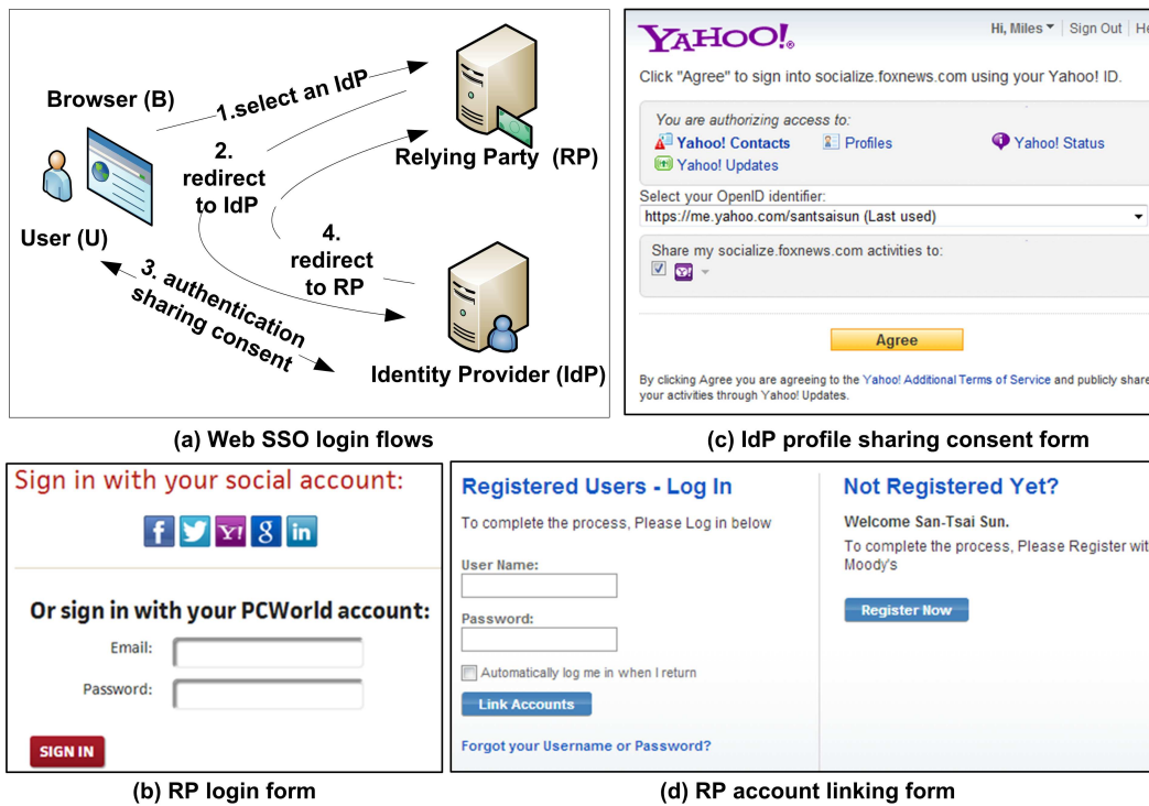
Fig. 1. Sample forms in web SSO sign-up and sign-in processes.
