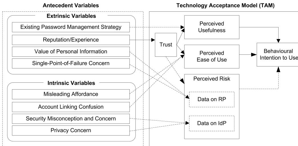
Fig. 12. Web single sign-on technology acceptance model. The acceptance factors we found are correlated as antecedent variables to the intermediate factors in TAM, and categorized as intrinsic and extrinsic variables. Solid arrowed lines indicate positive influences, while dashed arrowed lines represent negative influences.
