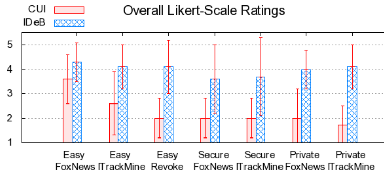
Fig. 5. The overall Likert-scale ratings from post-condition questionnaires in the formative study.
