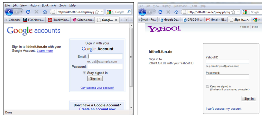
Fig. 3. Screen shots of the IdP phishing demo website.
